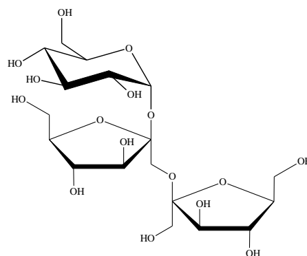
(O-β-D-fructofuranosyl-(2-1)-β-D fructofuranosyl-(2-1)-α-D-glucopyranoside)
